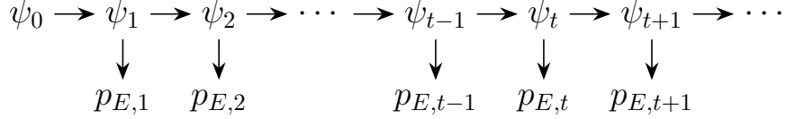
Figure D.27: Acyclic directed graph of the state-space model
